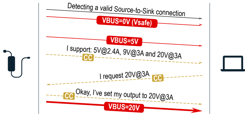
Powering Handshake
