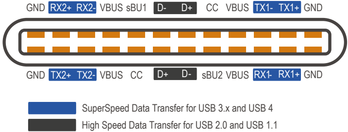
The pinout of the USB-C connector
