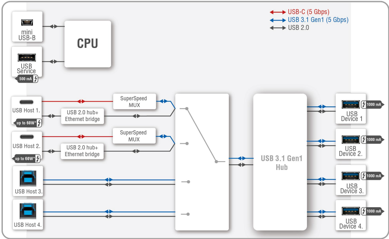
USB Port Diagram (UCX-4x2-HC30D)
